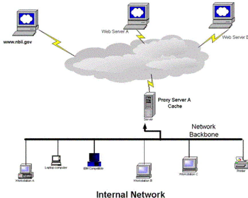
Figure 1a: Proxy Server.
